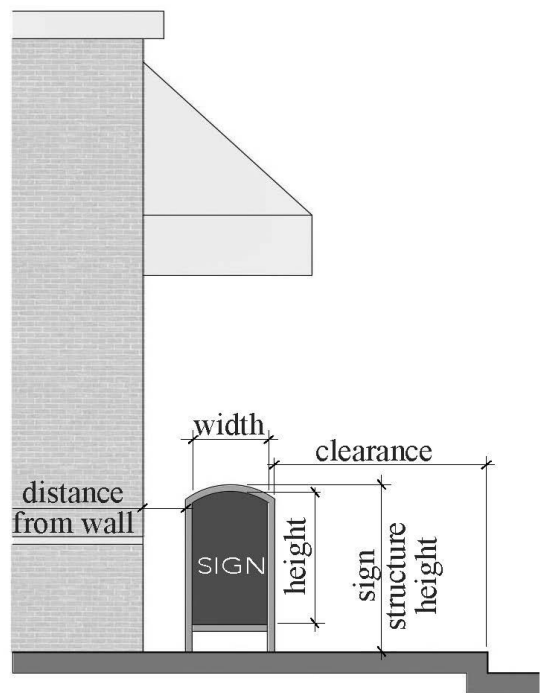
Figure 7.23 Sidewalk sign detail
